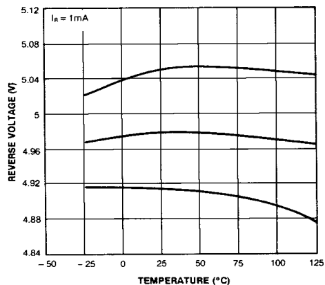
Figure 2. Temperature Drift
